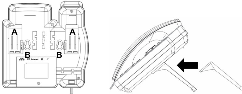
Figure 2-3: Desktop Mounting
