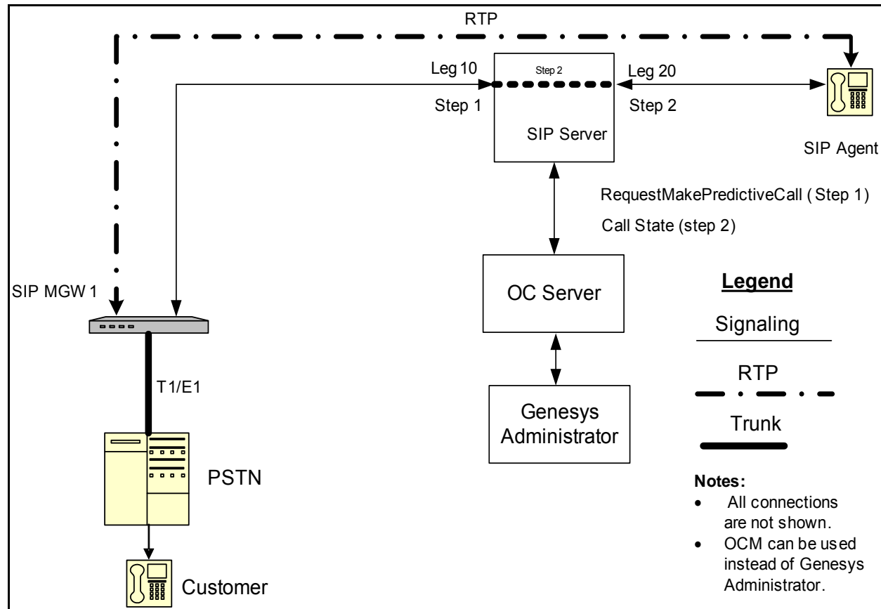
Figure 10: Transfer-Mode Call Flow (MGW with CPA) with a SIP Agent Endpoint
