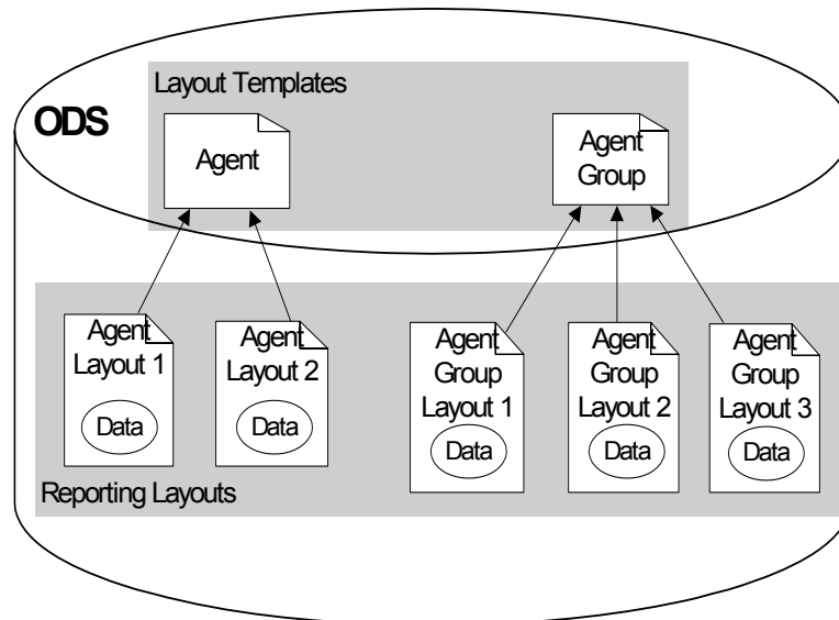
Figure 79: Layouts and Templates
