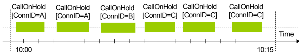
Figure 71: Using DistByConnID Qualifier
