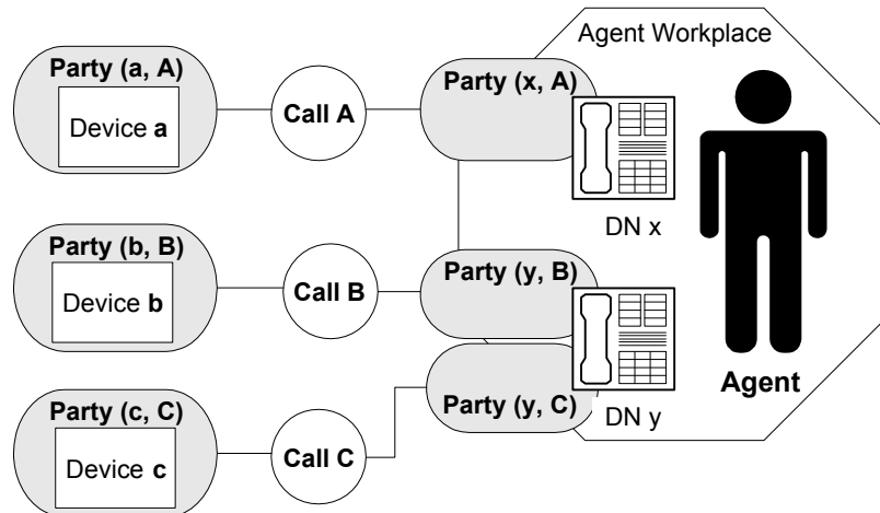
Figure 18: Agent's Environment
