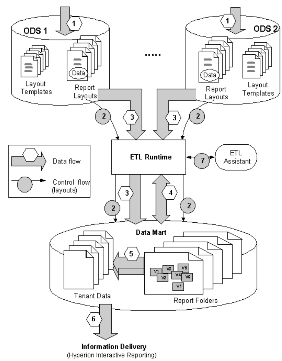
Figure 81: Data Aggregation
