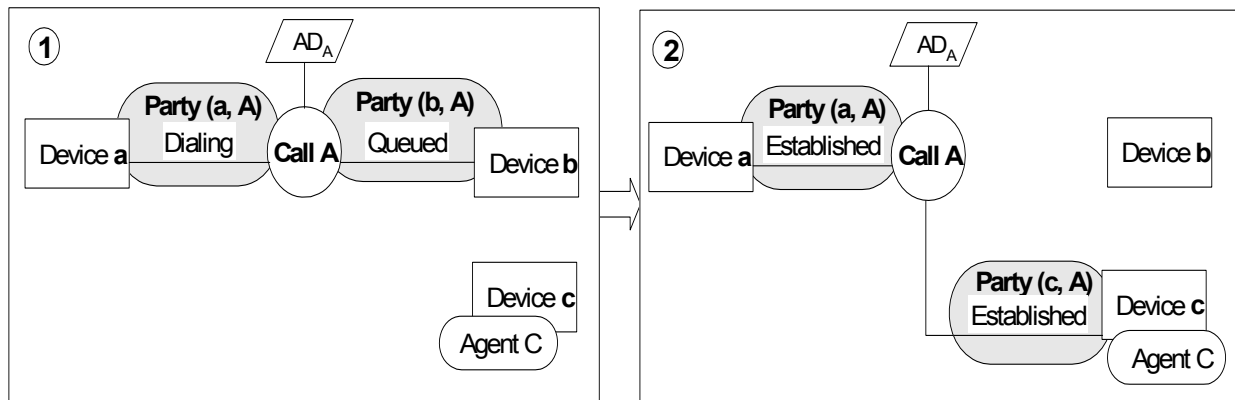
Figure 27: Call-Routing Scenario
