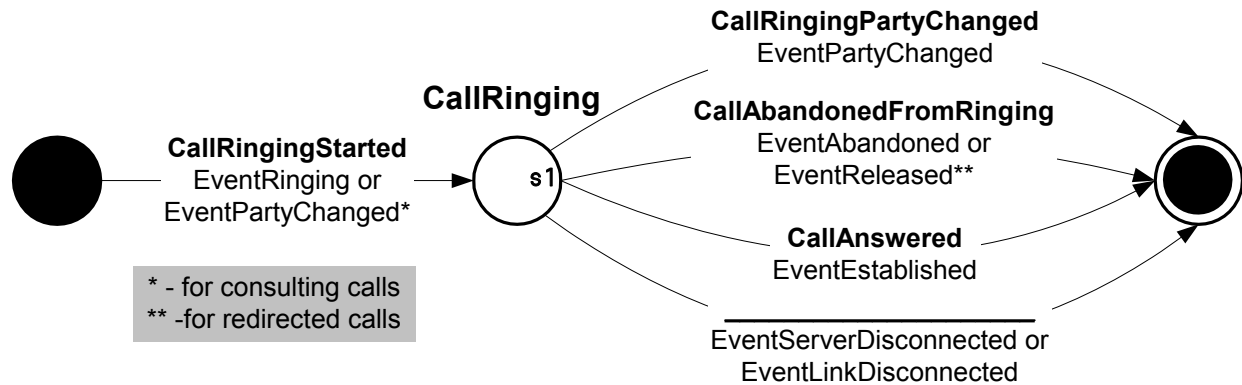
Figure 56: CallRing Action
