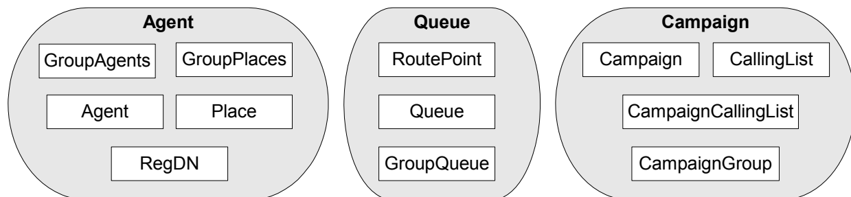
Figure 64: Partitioning Objects into Compatibility Groups
