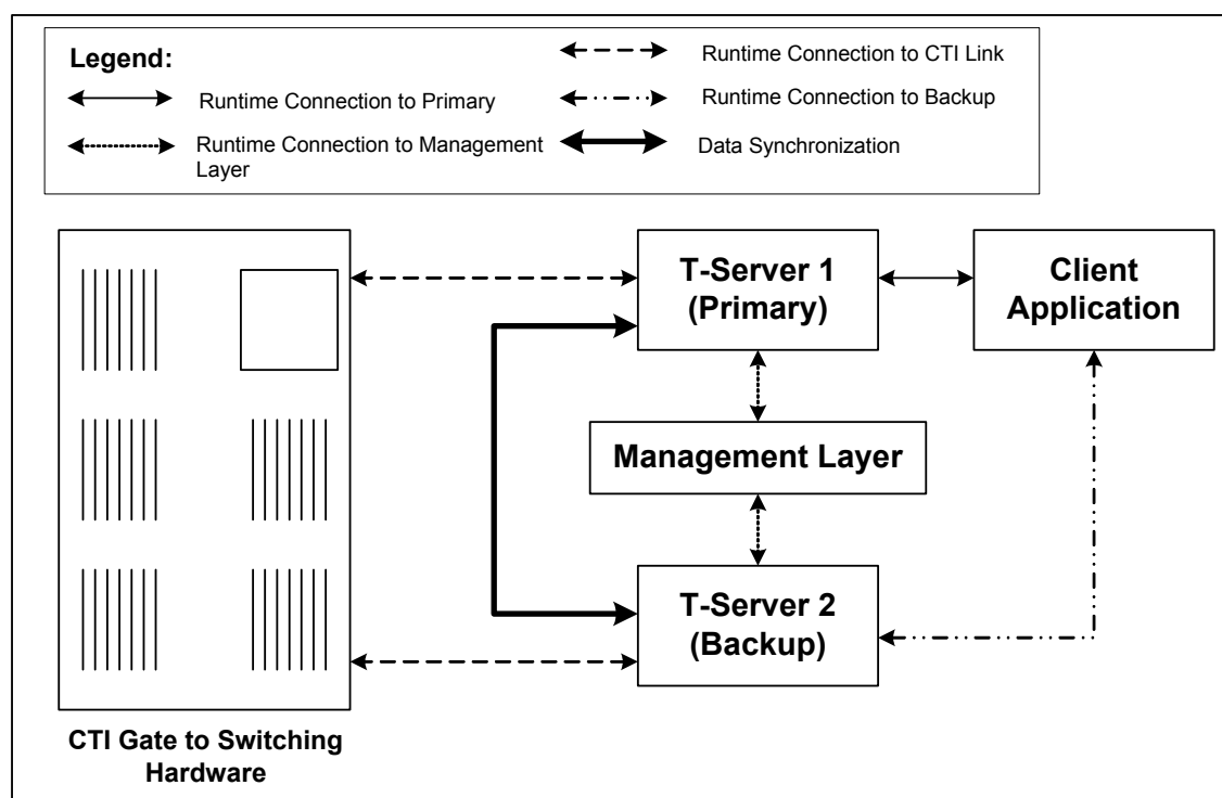
Figure 12: Hot Standby Redundancy Type Dual for a Single CTI Link with Two T-Servers
