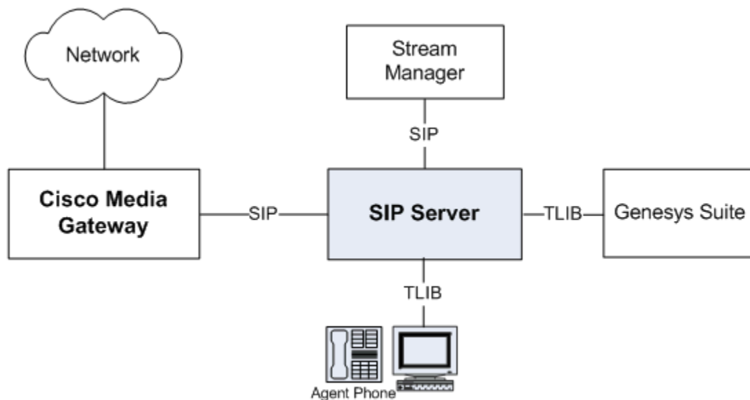
SIP Server - Cisco Media Gateway Deployment Architecture
