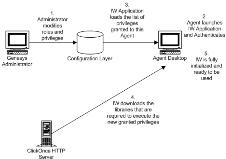
Update of the agent's role through ClickOnce (IW = Interaction Workspace)
