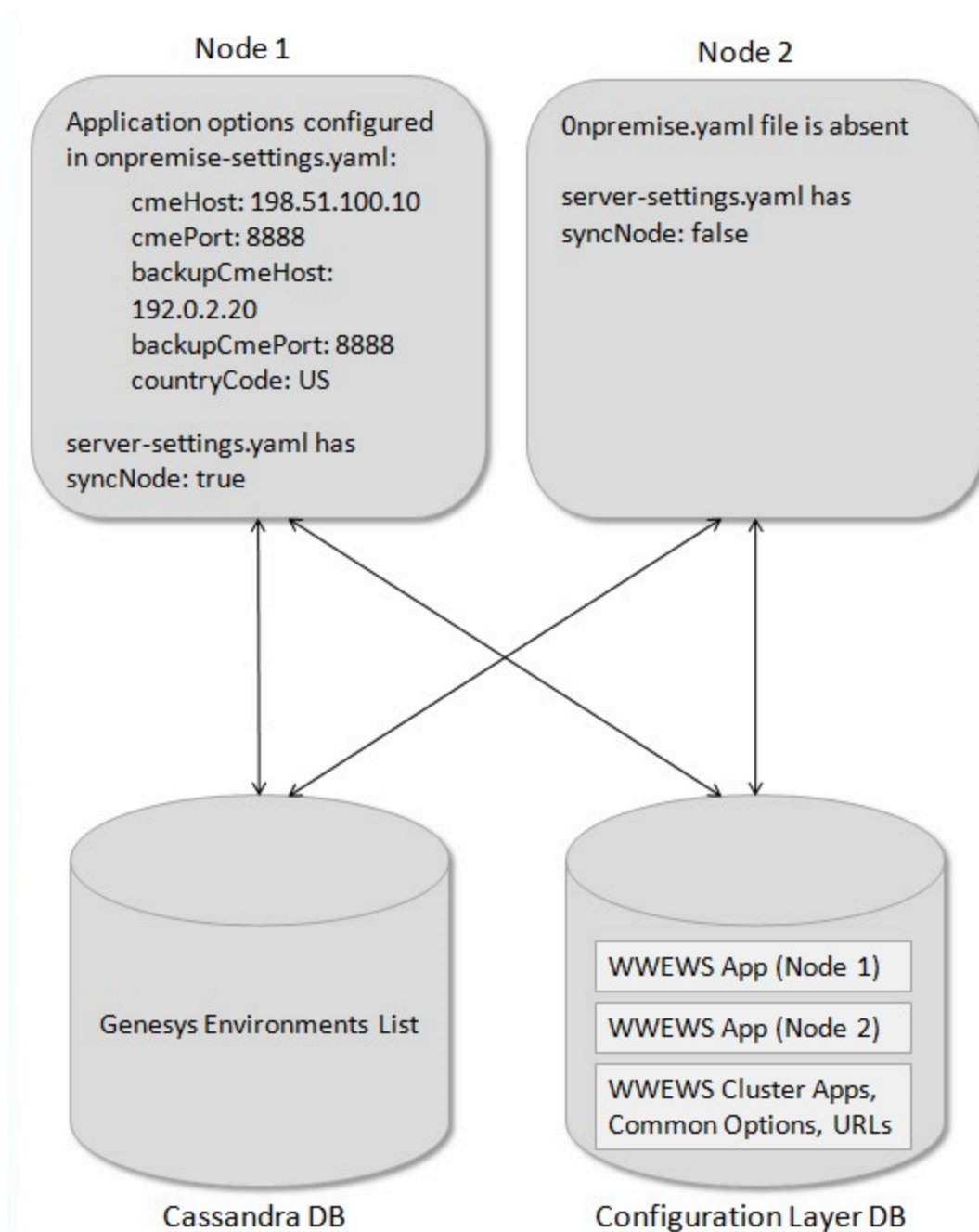
Workspace Web Edition &amp; Web Services On-Premise Architecture
