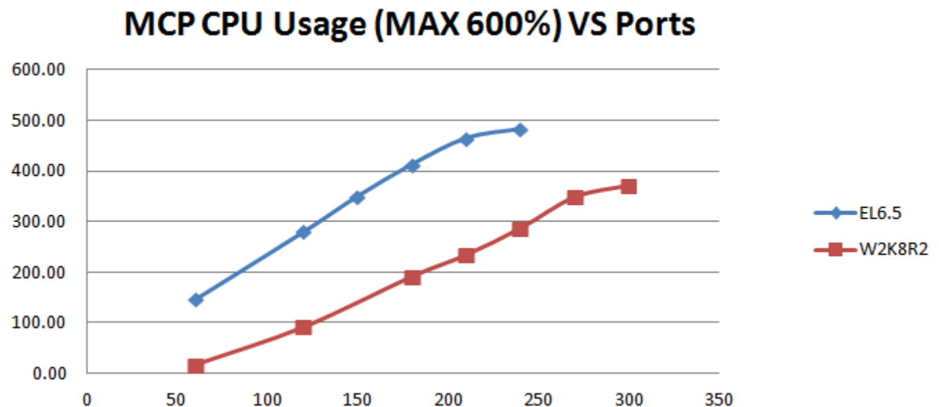
Figure 74: Comparison of MCP CPU Usage on a physical server, MP3 16kbps without encryption, RH EL 6.5 vs. Windows 2008 R2
