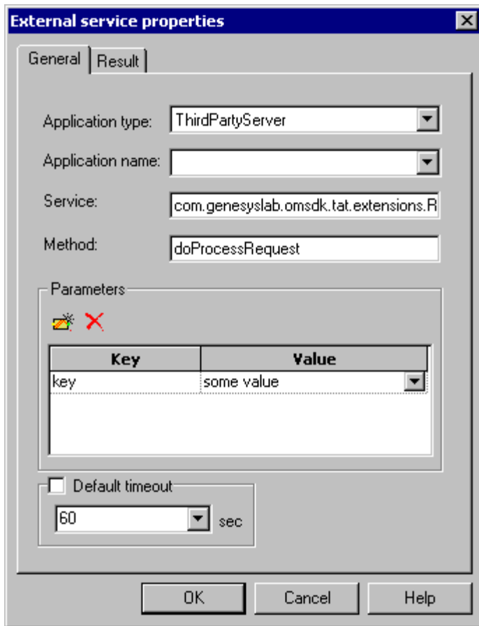
External Service Properties Window
